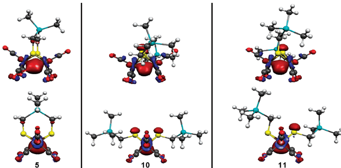
Figure 7. Orbital surfaces (value = \pm 0.05 ) for the HOMOs of 5 , 10 , and 11 .
